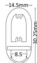
ICR-B Illuminated Coat Rail - Black
